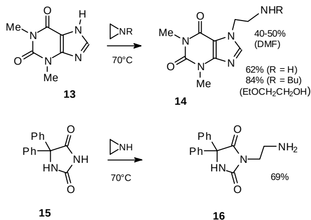
Scheme 4 NRO of Aziridine Bases by SH Compounds and by Acidic NH Compounds
