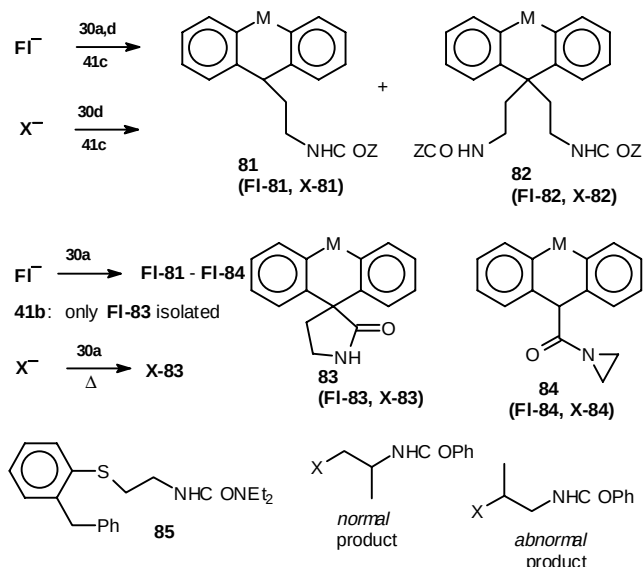
Scheme 15 Unhindered NRO of N -Acylaziridines by Diarylmethanide Anions
