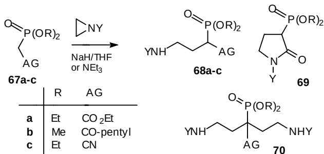
Scheme 12 C-Amidoethylation of Horner Reagents
