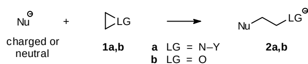
Scheme 1 Nucleophilic Ring Opening of three-membered Rings
