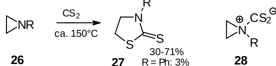
Scheme 6 CS 2 as Lewis Acid and Reactant for N -substituted Aziridine Bases
