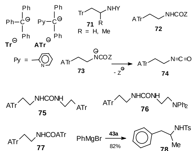
Scheme 13 Reactions of Activates Aziridines with Triaryl-methanide Ions and with Phenylmagnesium Bromide
