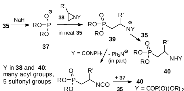
Scheme 8 P-Amidoethylation of Dialkylphosphite Anions
