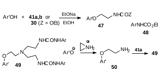
Scheme 10 Reactions of N-Acylaziridines with Phenolates
