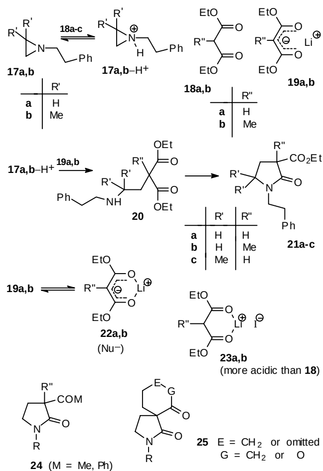
Scheme 5 C-Aminoethylation of \beta -Dicarbonyl Compounds
